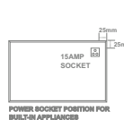
POWER SOCKET POSITION FOR BUILT-IN APPLIANCES
